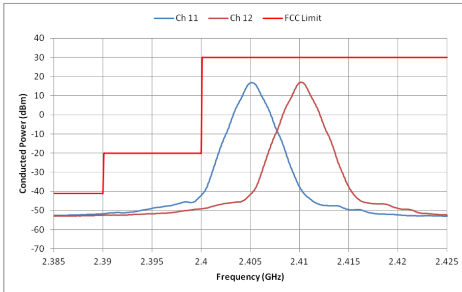
Figure 9. Conducted Spurious Emission, Lower Band Edge (TXPOWER = 0xE5, RBW = 1 MHz, VBW = 10 Hz)
