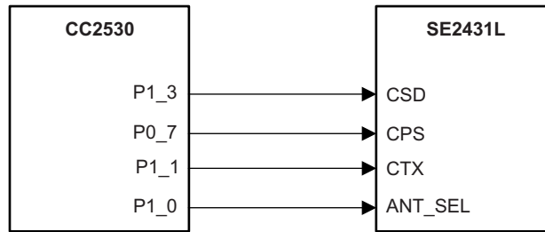
Figure 11. CC2530-SE2431L Interconnect
