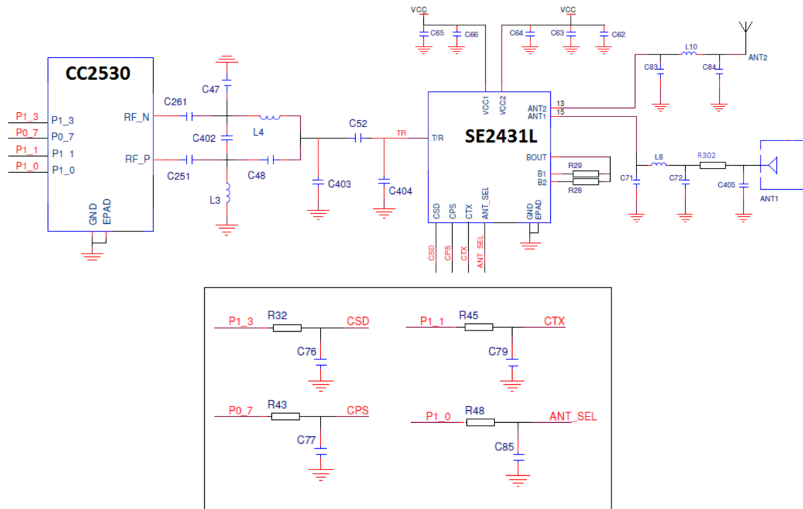
Figure 7. Application Circuit for the CC2530 With SE2431L
