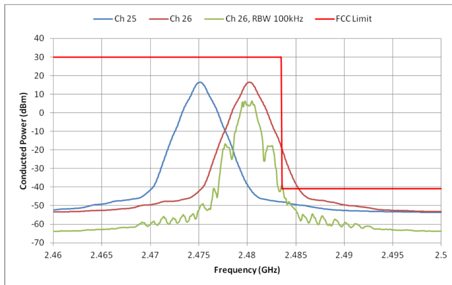
Figure 10. Conducted Spurious Emission, Upper Band Edge (TXPOWER = 0xE5, RBW = 1 MHz (100 kHz), VBW = 10 Hz)
