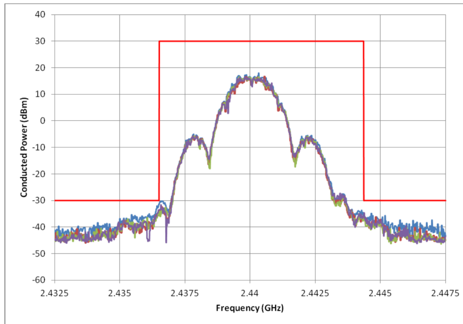
Figure 6. Conducted Power Spectral Density, TXPOWER = 0xF5
