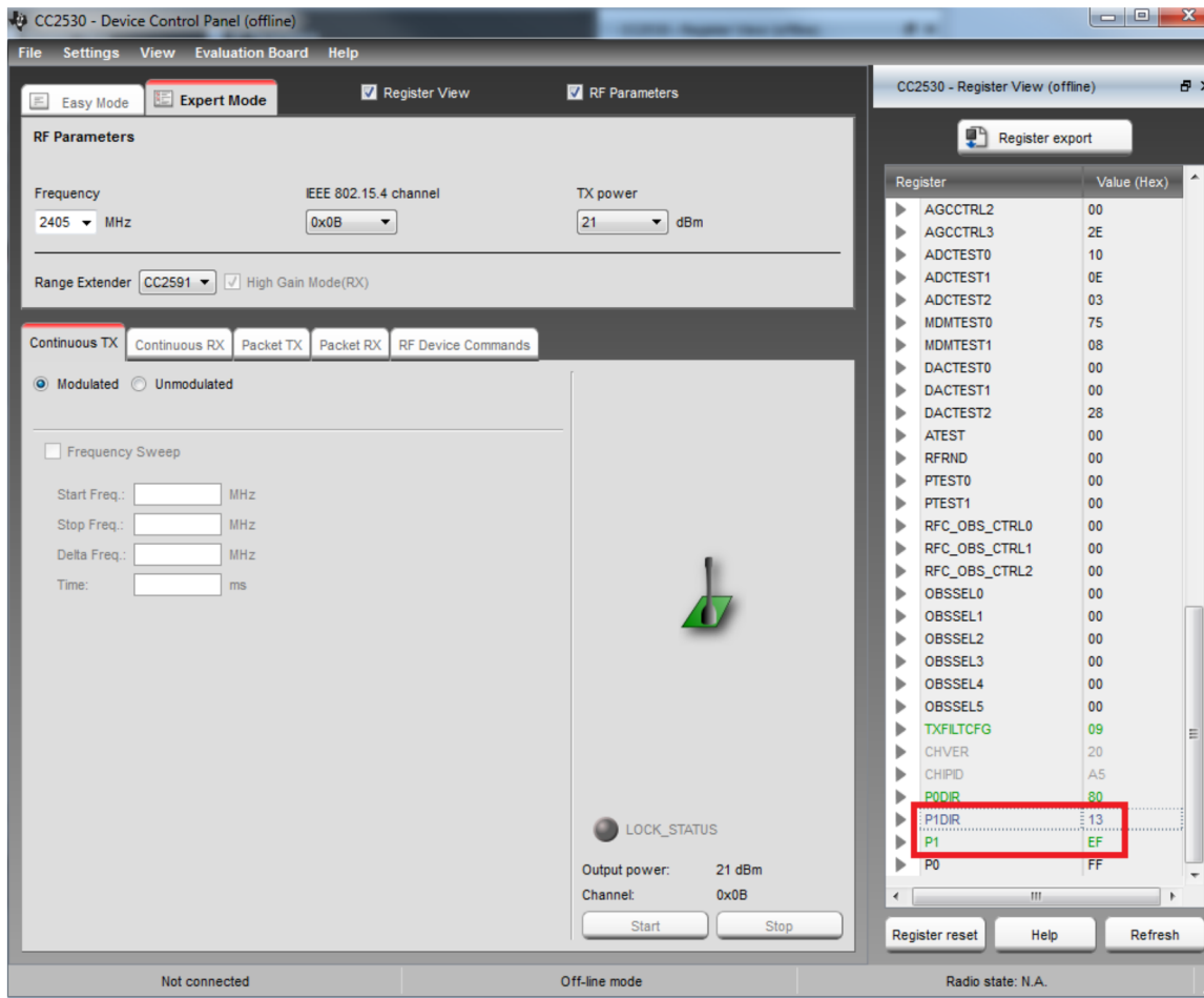
Figure 12. CC2530-SE2431L Interconnect Register Settings
