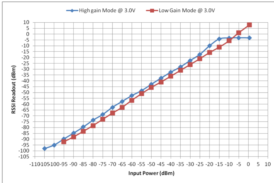
Figure 5. RSSI Readout vs. Input Power
