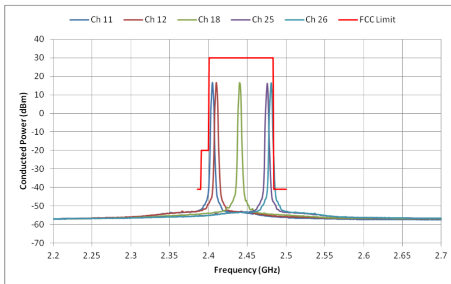
Figure 8. Conducted Spurious Emission vs. FCC Part 15.247 Limit (TXPOWER = 0xE5, RBW = 1 MHz, VBW = 10 Hz)
