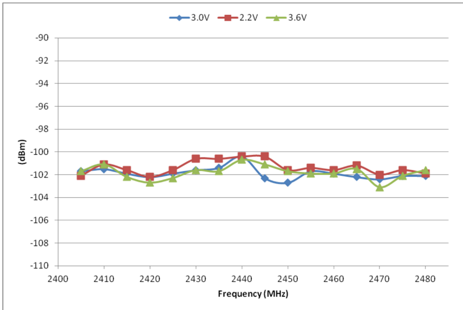
Figure 2. RX LNA Mode Sensitivity vs. Frequency and V_{DD}
