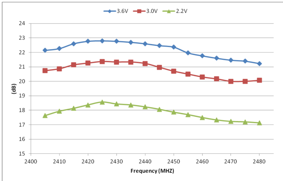
Figure 1. TX Power vs. Frequency and V_{DD} , TXPOWER = 0xF5
