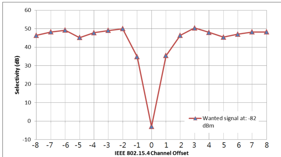
Figure 4. Selectivity Operating at Channel 18 (2440 MHz)
