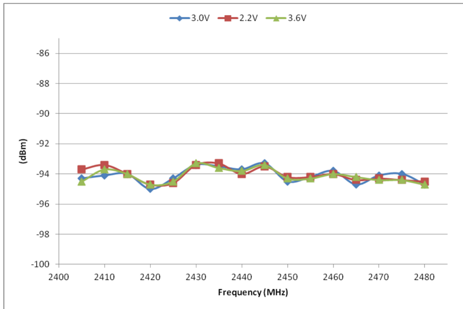
Figure 3. Rx Bypass Mode Sensitivity vs. Frequency and V DD
