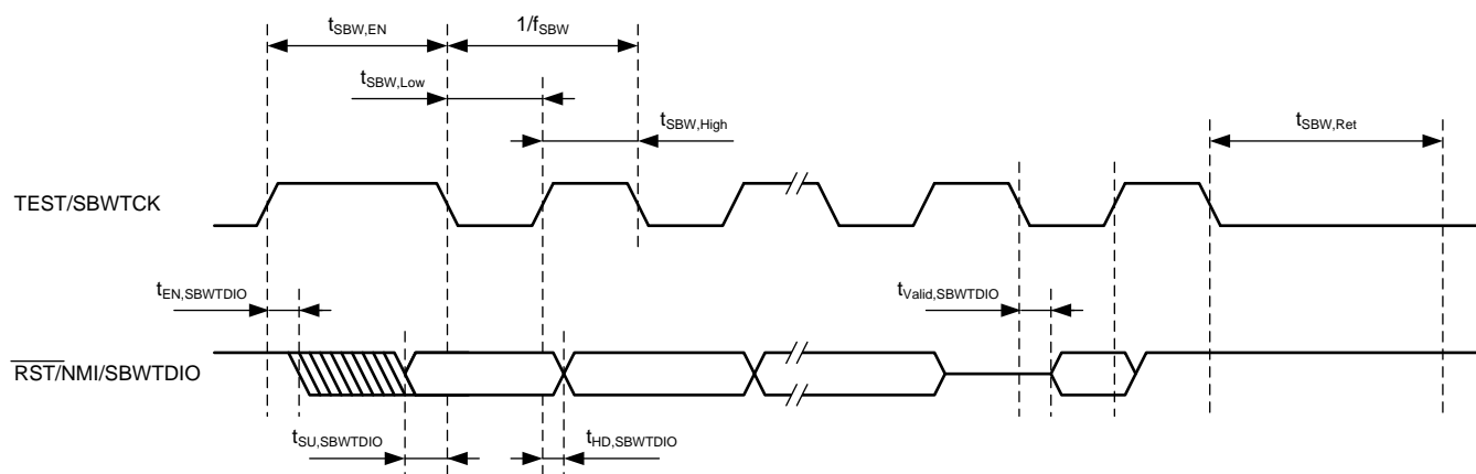
Figure 5-15. JTAG Spy-Bi-Wire Timing
