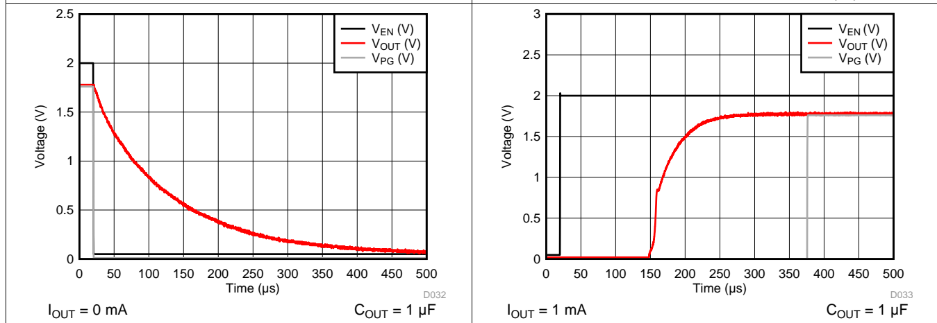
Figure 39. LP5912-1.8 V_{OUT} vs V_{EN(OFF)}
