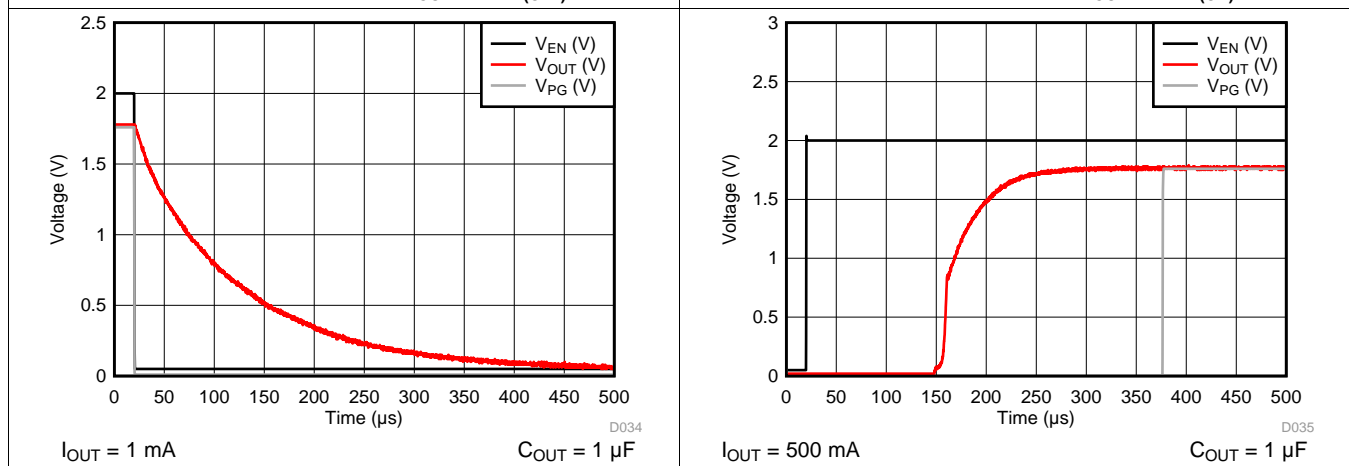
Figure 41. LP5912-1.8 V_{OUT} vs V_{EN(OFF)}
