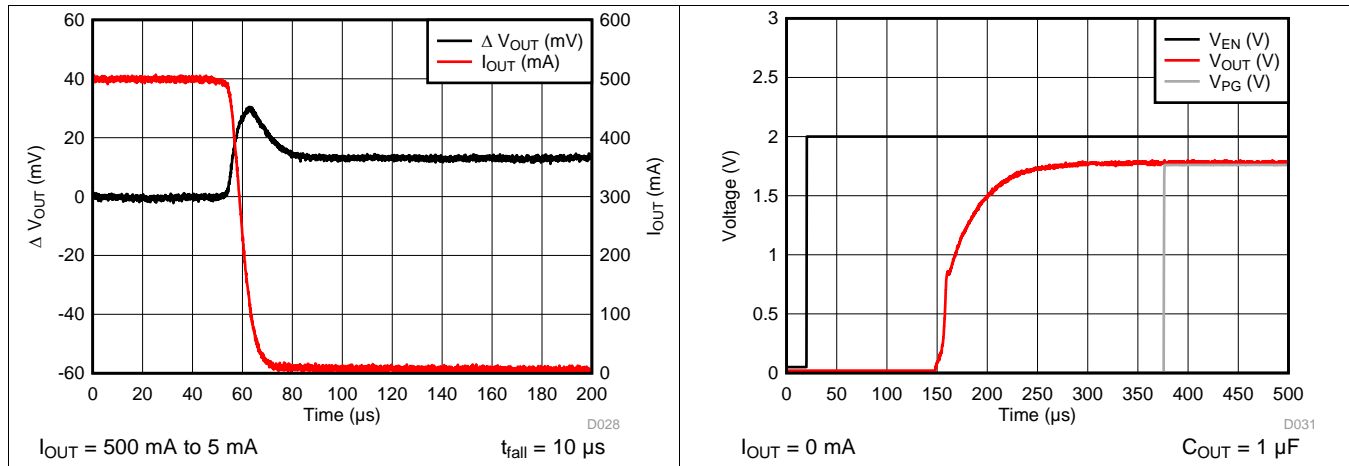
Figure 37. LP5912-3.3 Load Transient Response
