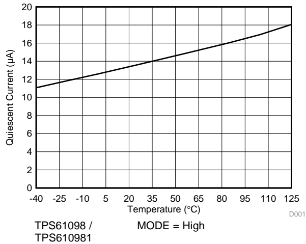
图 1. I_Q into VMAIN Pin at Active Mode vs Temperature
