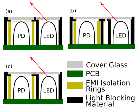
Figure 16. Cover glass design for flat cover glass
