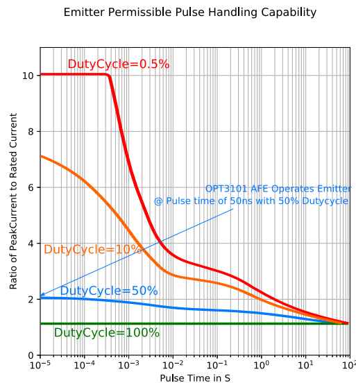
Figure 14. Duty Cycle Thermal Limit Curve for LED
