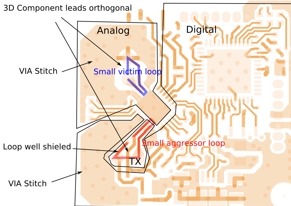
Figure 29. Good layout example 1
