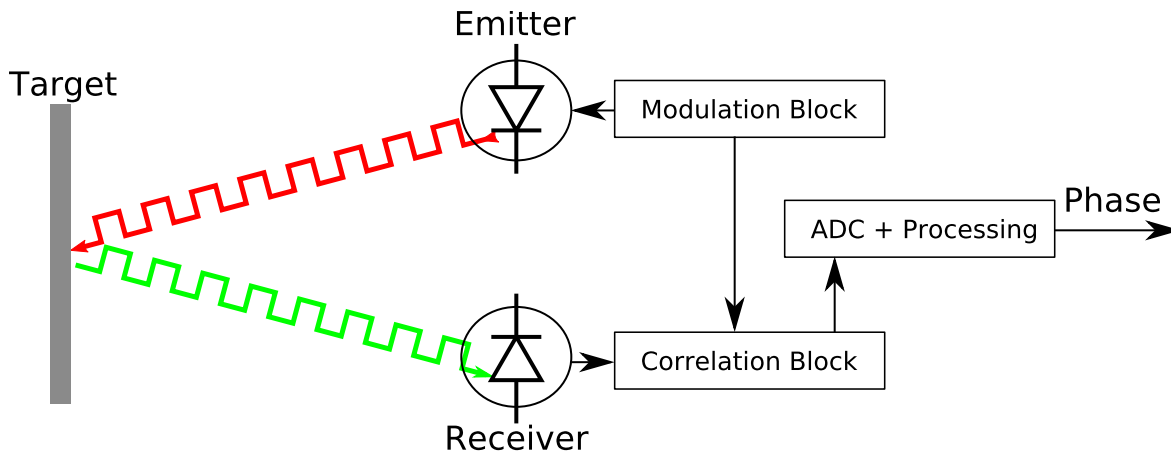
Figure 1. Generic ToF Proximity Sensor System
