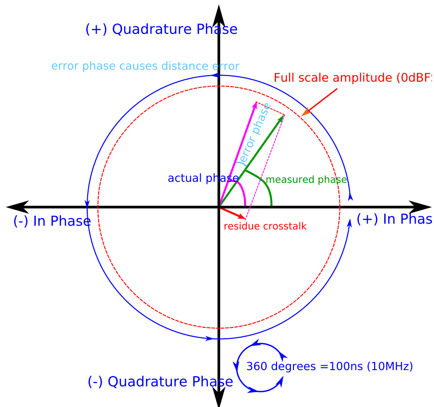
Figure 26. Vector diagram with residue crosstalk
