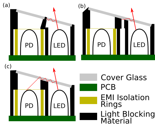
Figure 17. Cover glass design for angled glass
