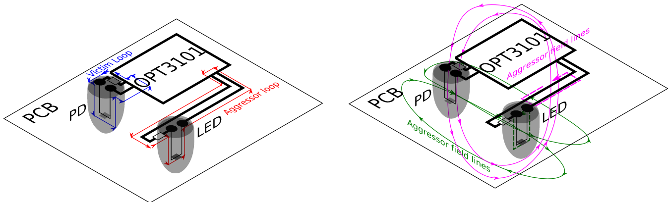
Figure 27. PCB Layout with magnetic field lines
