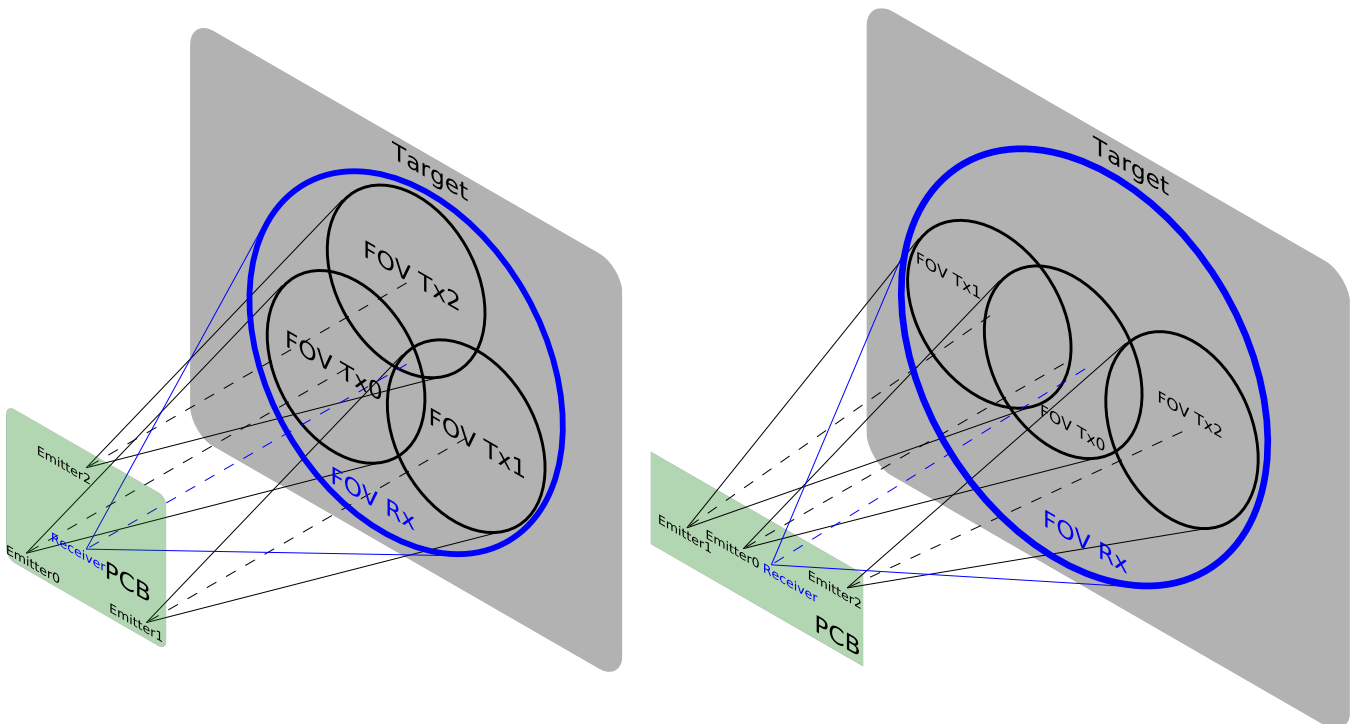
Figure 6. Multi-Zone Arrangement Examples With OPT3101
