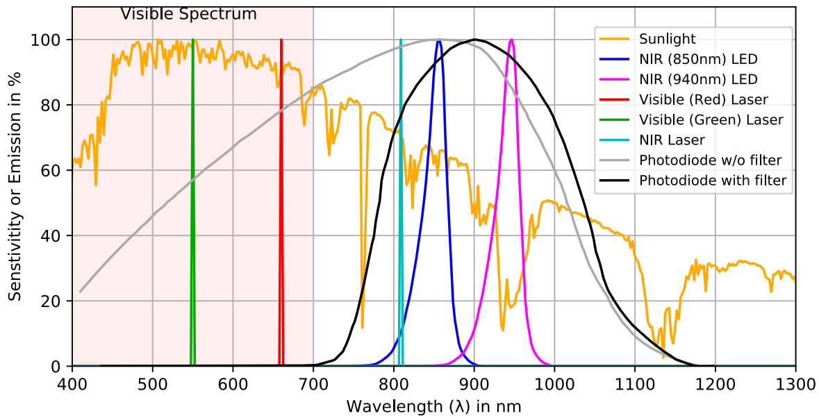
Figure 10. Spectral Response of Different Emitters and Photodiodes in Comparison With Solar Spectrum
