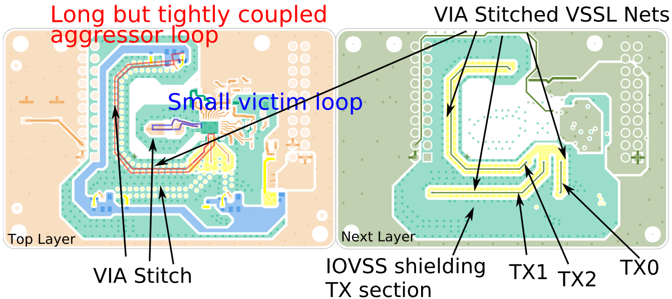
Figure 31. Good layout example 2
