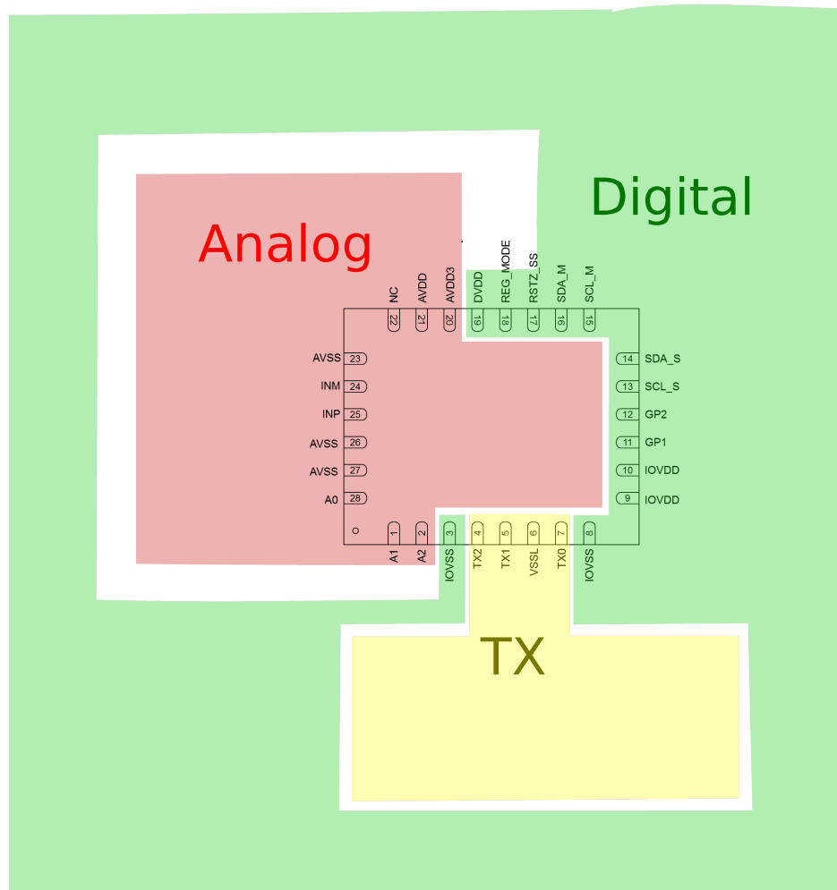
Figure 28. PCB sections recommended
