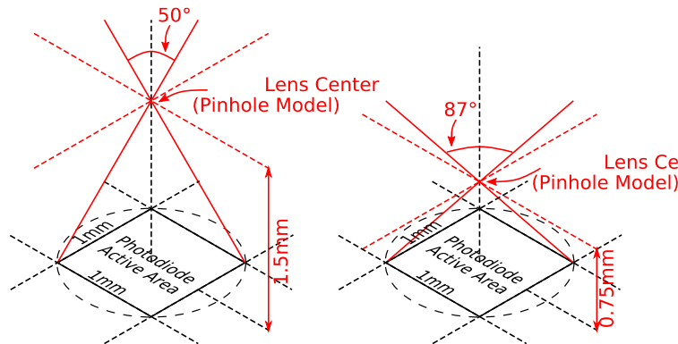
Figure 23. Field of View with pin hole model
