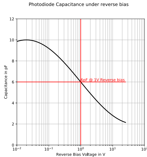
Figure 11. Reverse Biased Junction Capacitance Curve of Photodiode
