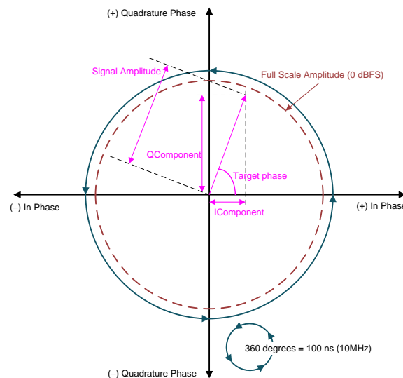
Figure 3. Vector Diagram Representation for ToF Signal
