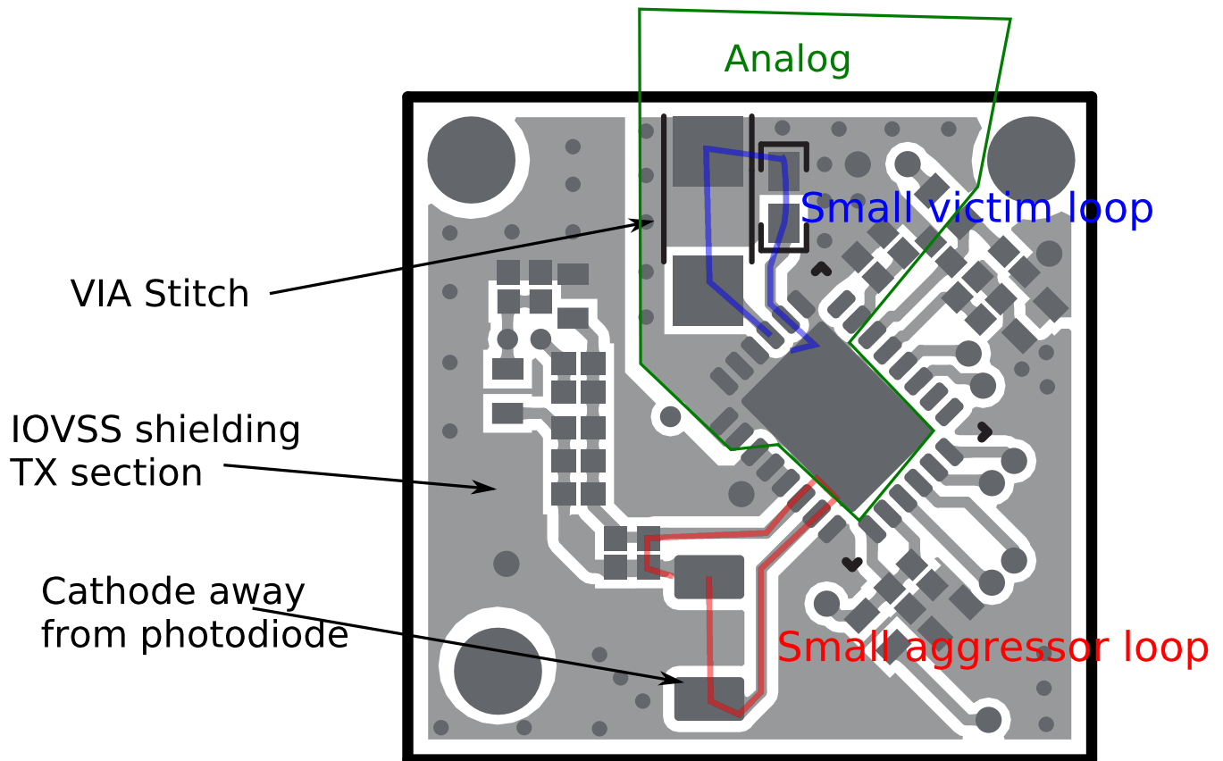
Figure 30. Good layout example 2
