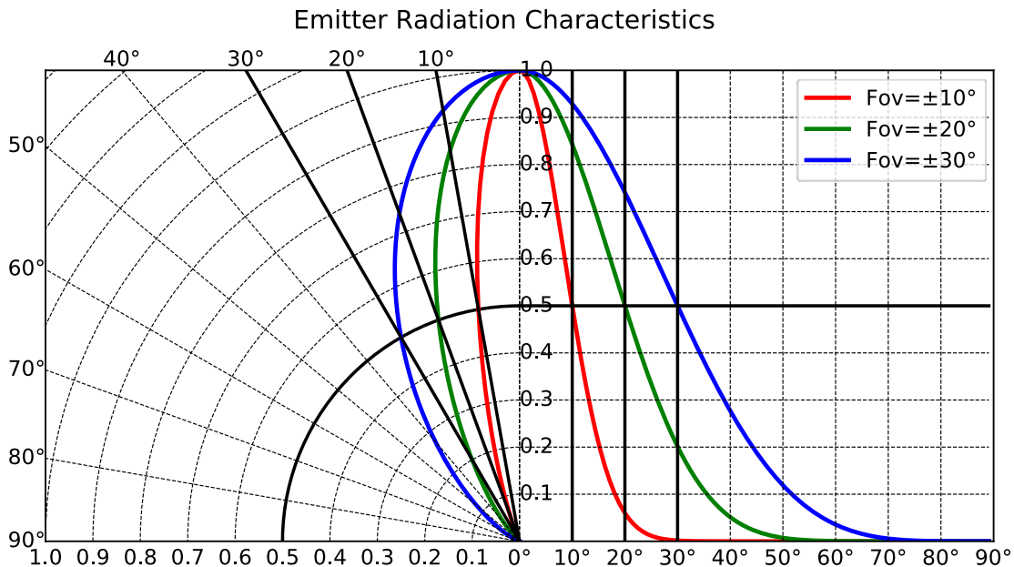
Figure 13. Angular Emissions of LEDs With Various FoVs
