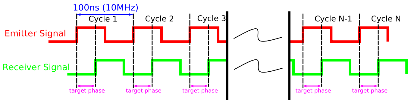
Figure 2. Generic Time-of-Flight Timing Diagram
