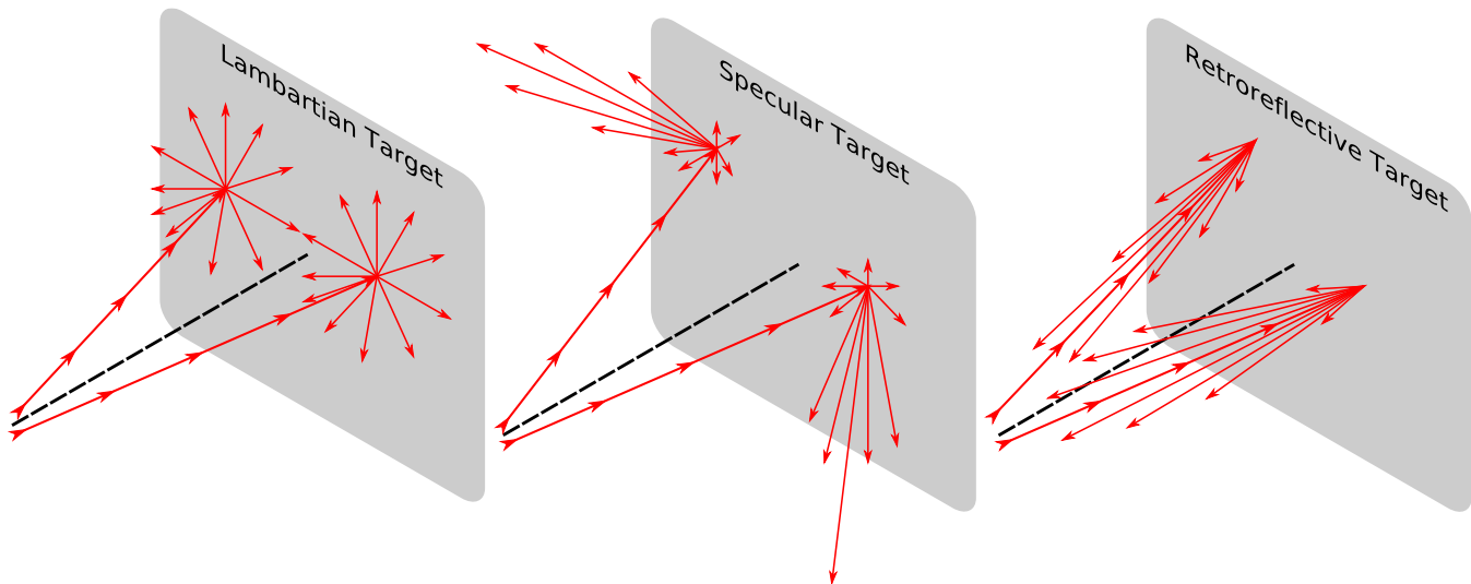
Figure 8. Type of Targets Based on Reflectance
