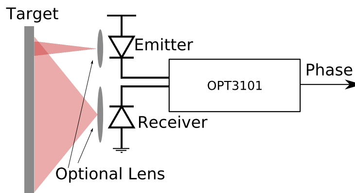
Figure 4. OPT3101-Based System
