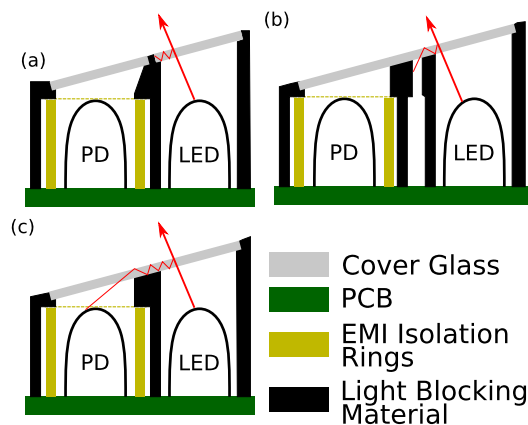
Figure 18. Cover glass design for angled glass
