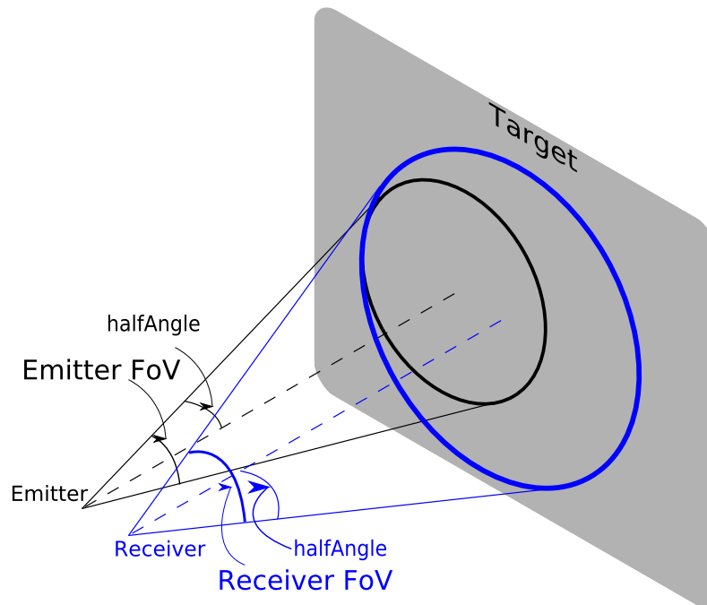
Figure 7. Emitter and Receiver Fields-of-View
