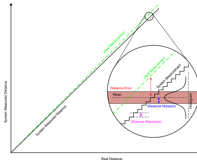
Figure 9. Performance Target Definitions
