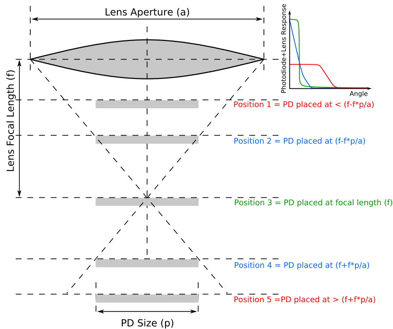
Figure 21. photodiode positioning from lens
