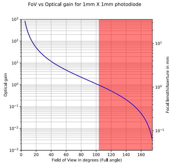
Figure 24. Field of view vs optical gain
