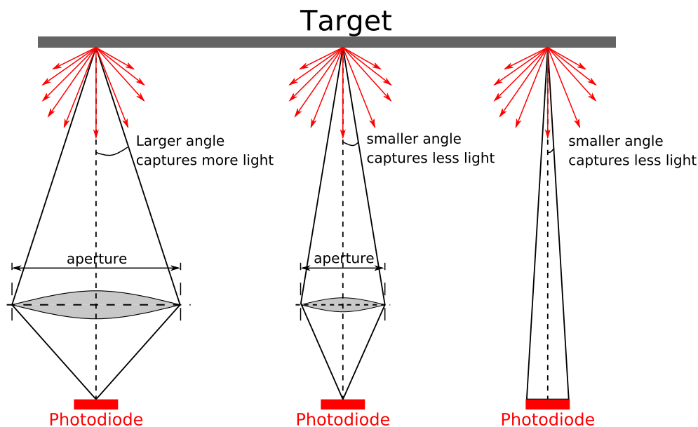
Figure 20. Receiver Optics with and without Lens
