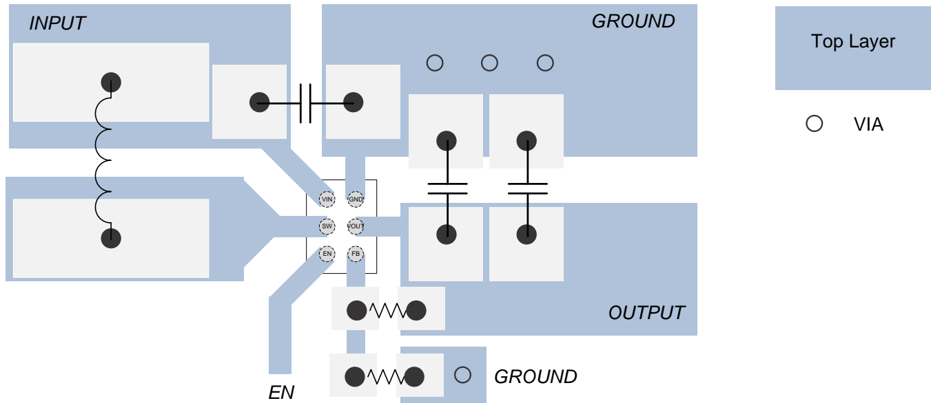
Figure 29. Layout -YFF
