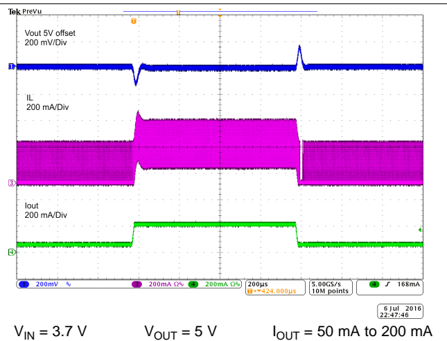
Figure 26. Load Transient
