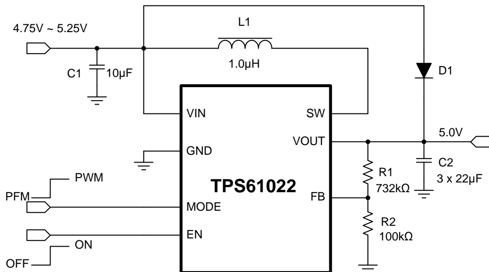
图 28. TPS61022 Circuit for V_{IN} > 4.8\text{-V} Application
