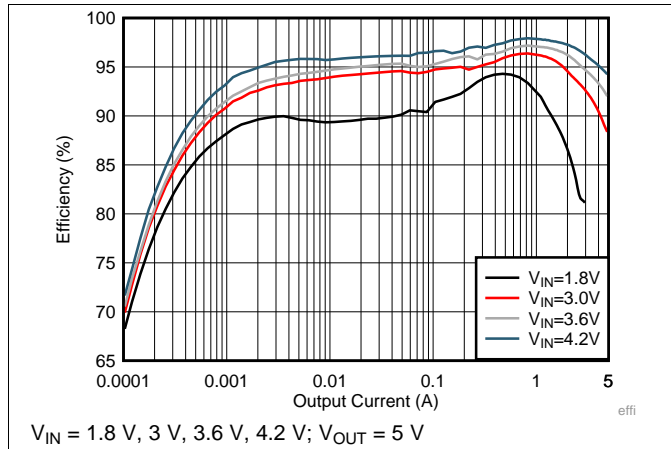
图 1. Load Efficiency With Different Input in Auto PFM
