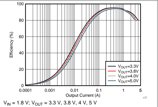
图 2. Load Efficiency With Different Output in Auto PFM
