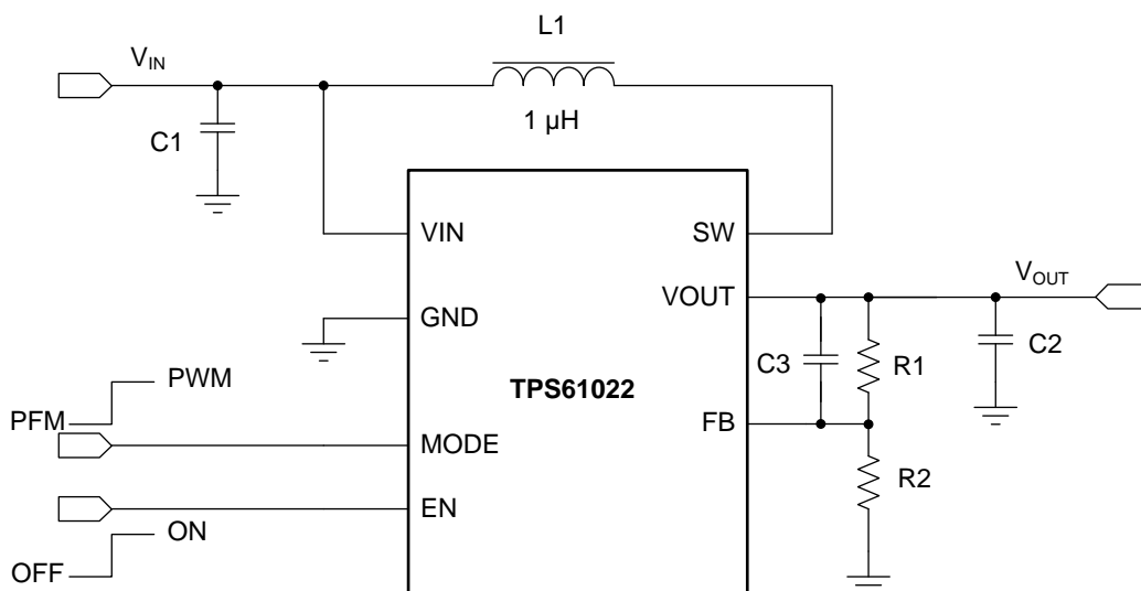
图 17. TPS61022 Circuit With Feedforward Capacitor
