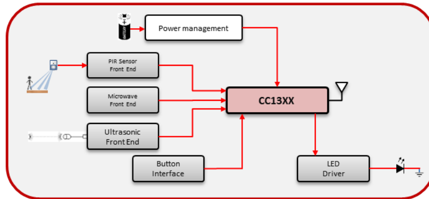
Figure 1. Motion Detection System Block Diagram
