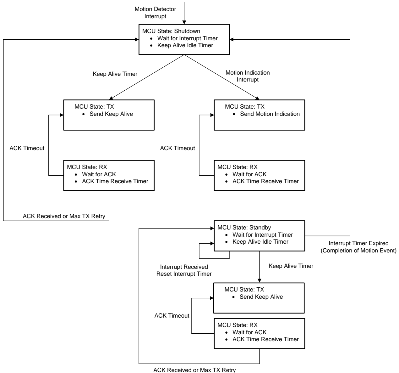
Figure 4. Test-Case State Machine
