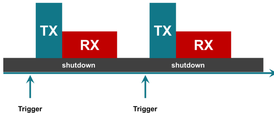
Figure 2. Power Profile
