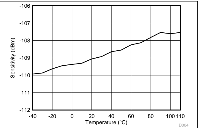
Figure 5-14. RX (50 kbps) Sensitivity vs Temperature 915 MHz
