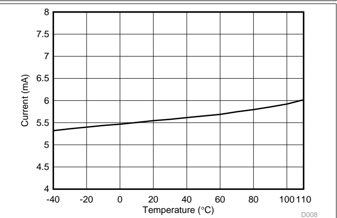
Figure 5-18. RX (50 kbps) Current vs Temperature at 915 MHz
