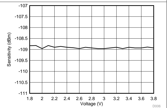
Figure 5-16. RX (50 kbps) Sensitivity vs Voltage 915 MHz
