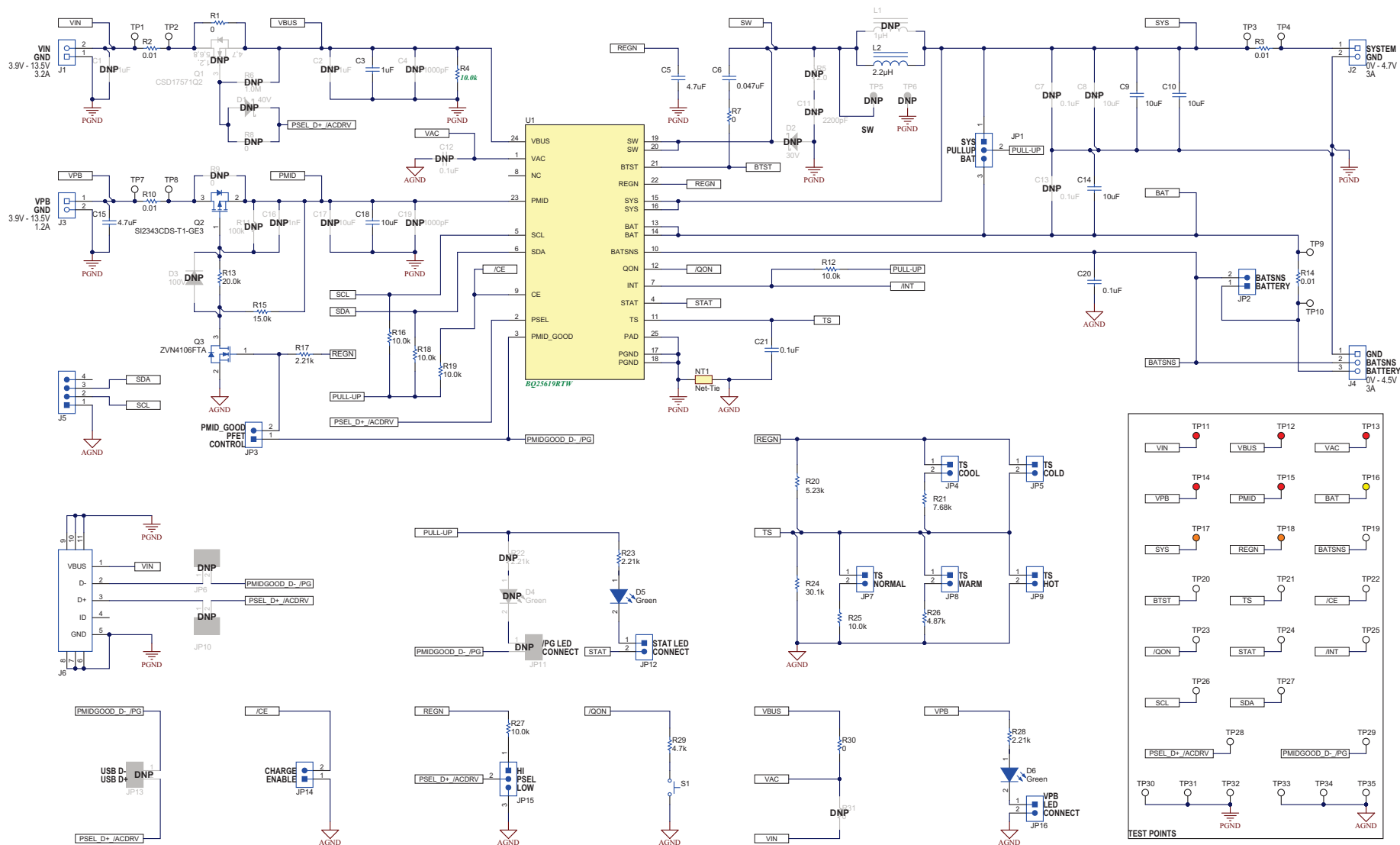
Figure 15. BQ25619EVM Schematic
