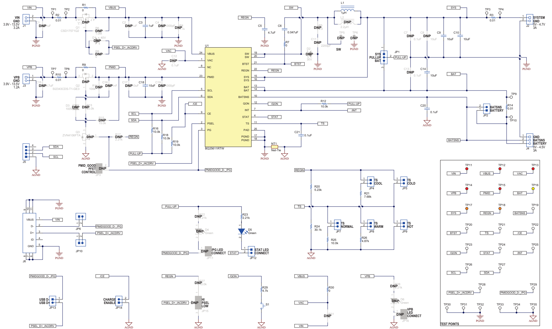
Figure 16. BQ25611DEVM Schematic
