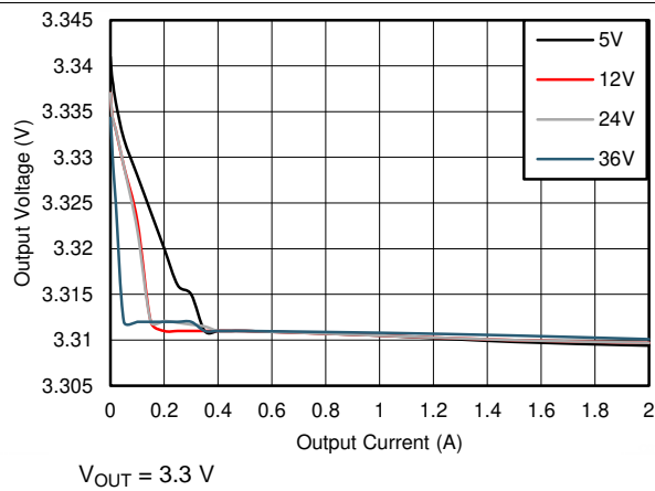
图 44. Line and Load Regulation
