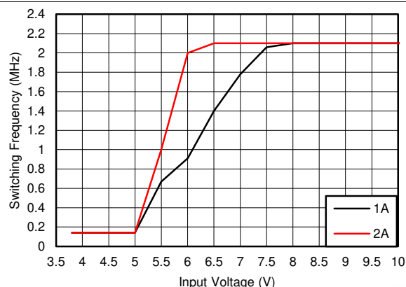
图 18. Typical Switching Frequency in Dropout Mode V_{OUT} = 5\text{ V} , f_{SW} = 2.1\text{ MHz}
