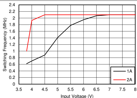
图 17. Typical Switching Frequency in Dropout Mode V_{OUT} = 3.3\text{ V} , f_{SW} = 2.1\text{ MHz}
