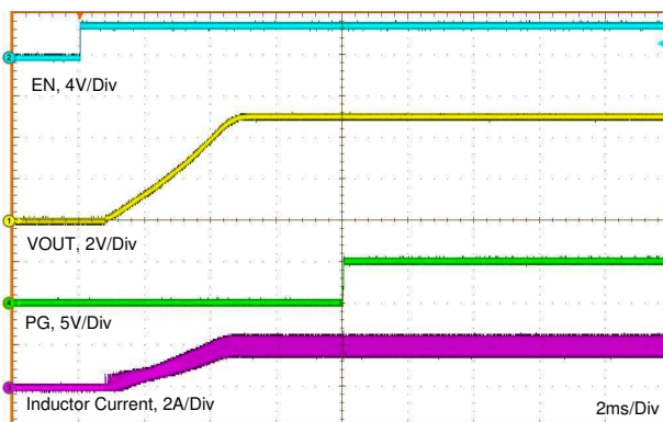
图 10. Typical Start-up Behavior V_{IN} = 12\text{ V} , V_{OUT} = 5\text{ V} , I_{OUT} = 2\text{ A}
