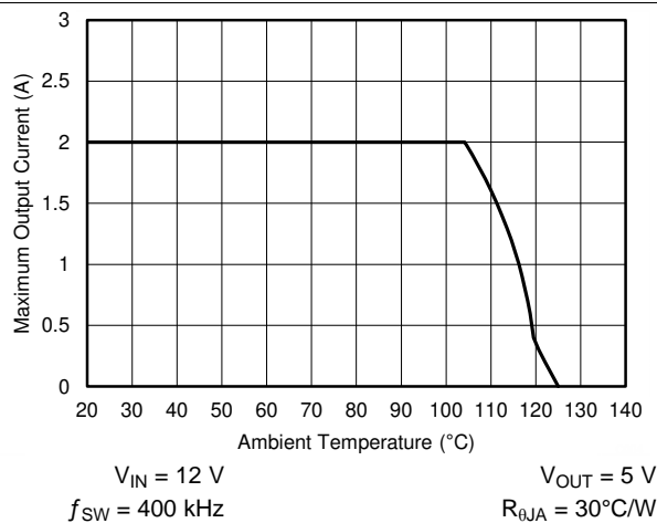
图 24. Maximum Output Current vs Ambient Temperature
