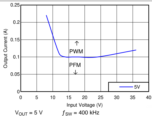
图 40. Mode Change Thresholds
