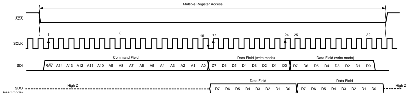
图 88. Serial Interface Protocol - Streaming Read / Write
